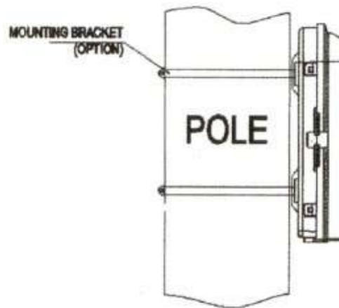
Pic 5 Pole mounted installation
