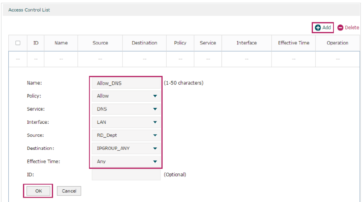
Figure 3-15 Configure Allow Rule for DNS Service
