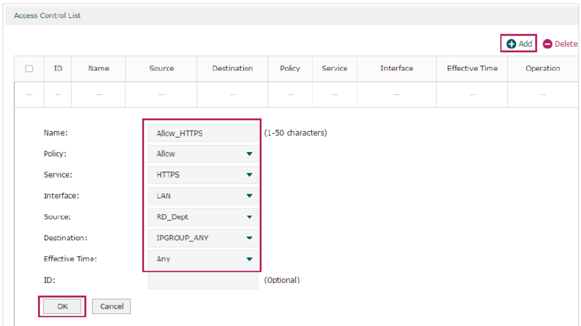
Figure 3-14 Configure Allow Rule for HTTPS Service
