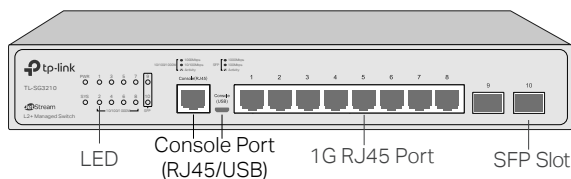
Figure 1-2 Front Panel of TL-SG3210
