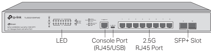
Figure 1-3 Front Panel of TL-SG3210XHP-M2
