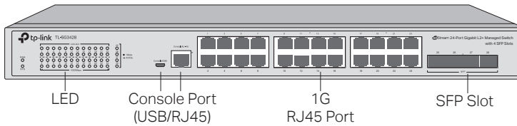
Figure 1-4 Front Panel of TL-SG3428 V2.0
