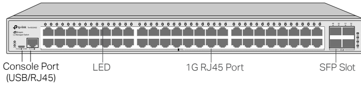
Figure 1-8 Front Panel of TL-SG3452
