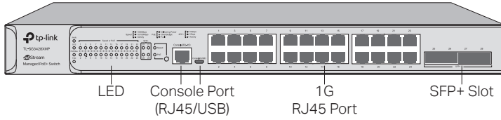
Figure 1-7 Front Panel of TL-SG3428XMP
