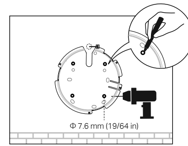
Plastic Wall Anchors
