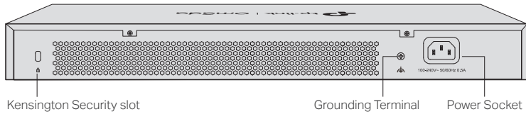
Figure 1-8 Rear Panel
