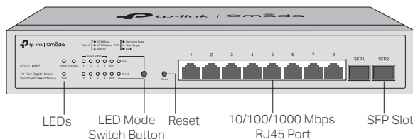
Figure 1-2 Front Panel of SG2210MP
