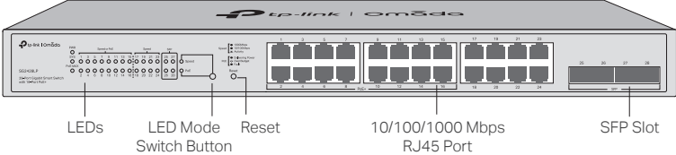
Figure 1-4 Front Panel of SG2428LP
